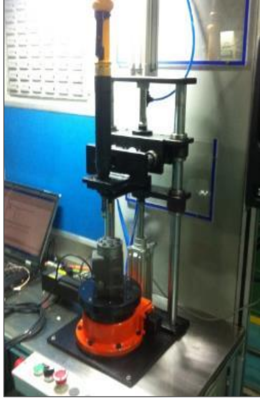
Bolting SPM
